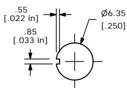
PANEL MOUNTING
