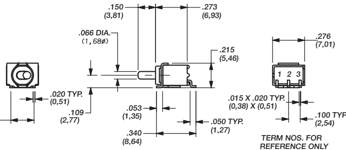
GT11MSABE Horizontal Actuation SPDT
