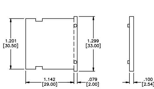
DPS910A2 Spacer
