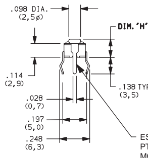
PTS453TL38 SPST
