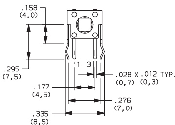
PTS645VJL61 SPST
