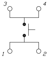
CIRCUIT: SPST CONTACT CONFIGURATION
