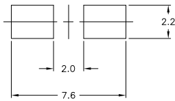
SOLDER LAND DIMENSION
