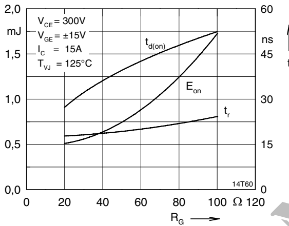
Fig. 9 Typ. turn on energy and switching
