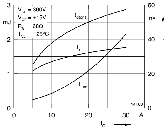
Fig. 7 Typ. turn on energy and switching
