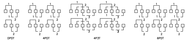
CIRCUIT DIAGRAMS
