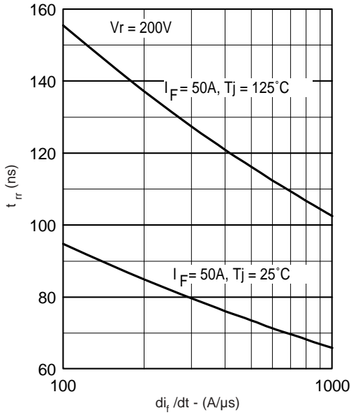
Fig. 6 - Typical Reverse Recovery vs. d i_t / d t
