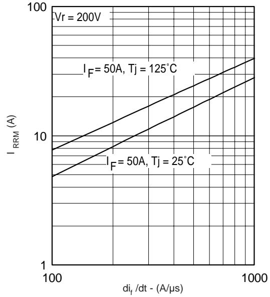
Fig. 7 - Typical Reverse Recovery Current vs. d i_t / d t
