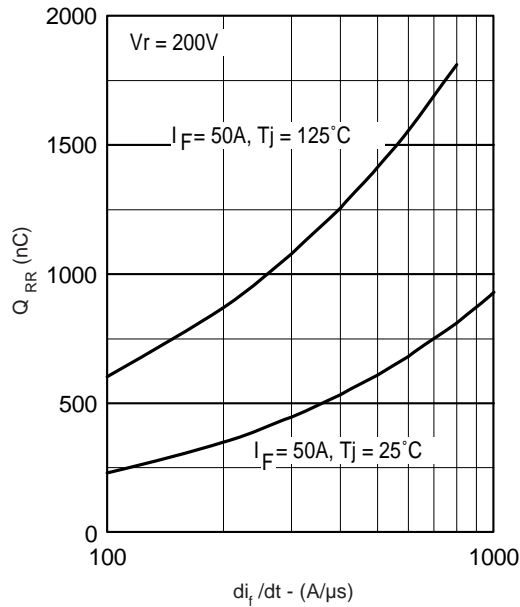
Fig. 8 - Typical Stored Charge vs. d i_t / d t
