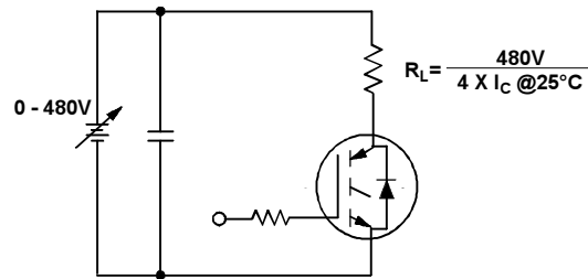
Figure 17. Pulsed Collector Current Test Circuit
