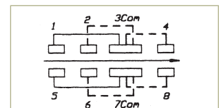
SCHEMATIC
