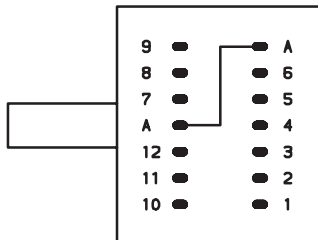
1 POLE 2 - 12 POSITIONS
