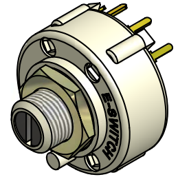
ISOMETRIC
