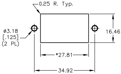
RECOMMENDED PANEL MOUNTING N.T.S.
