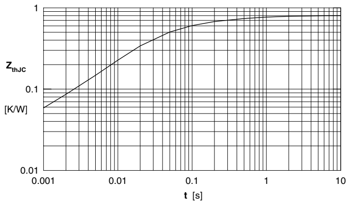
Fig. 2 Transient thermal impedance junction to case
