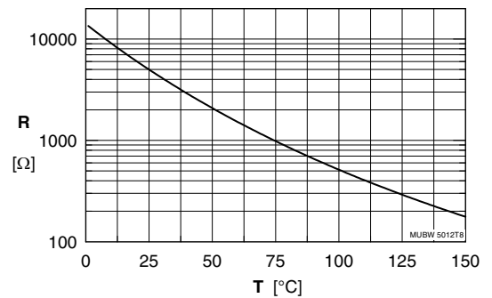
Fig. 15 Typ. thermistor resistance versus temperature
