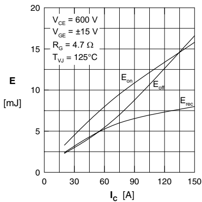
Fig. 7 Typical switching losses vs. collector current
