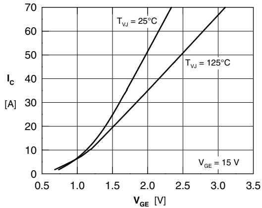
Fig. 10 Typical output characteristics
