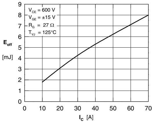
Fig. 12 Typ. turn off energy vs. collector current
