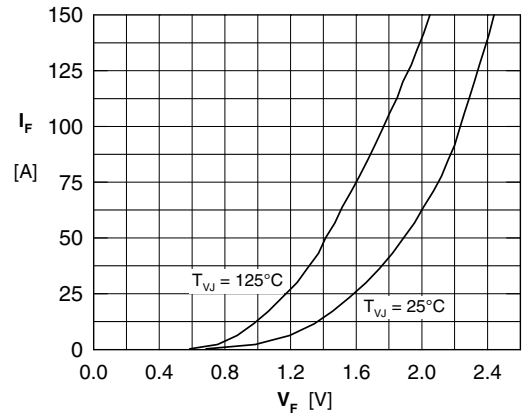
Fig. 6 Typical forward characteristic of free wheeling diode
