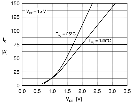
Fig. 3 Typical output characteristic
