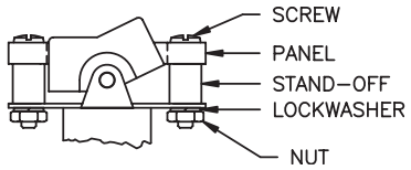
TYPICAL ASSEMBLY
