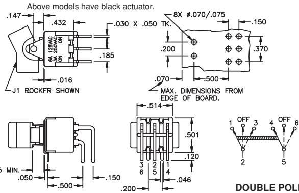
DOUBLE POLE
