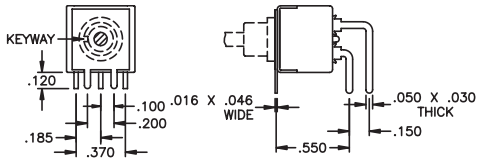
DOUBLE POLE HORIZONTAL P.C. MOUNTING
