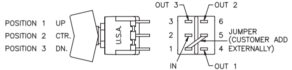
SIDE VIEW DOUBLE POLE
