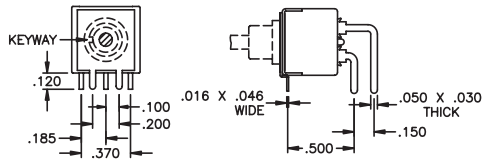
DOUBLE POLE HORIZONTAL P.C. MOUNTING
