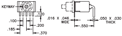
SINGLE POLE HORIZONTAL P.C. MOUNTING
