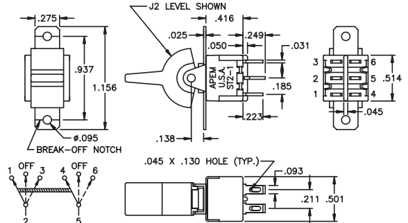
DOUBLE POLE
