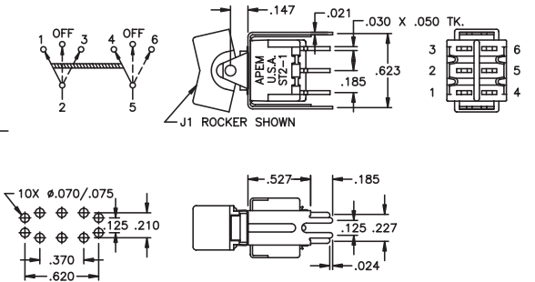
DOUBLE POLE
