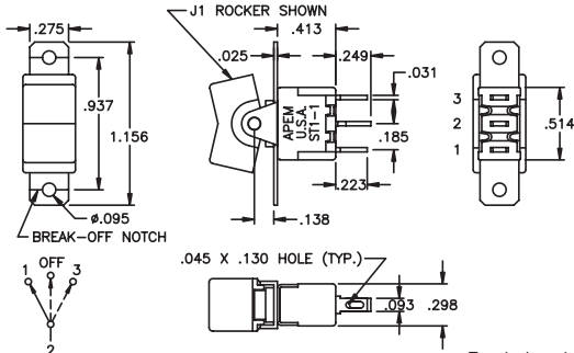
SINGLE POLE
