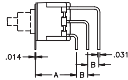
SIDE VIEW - SINGLE AND DOUBLE POLE
