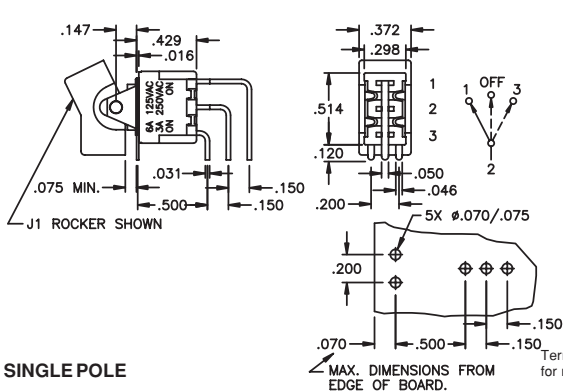
SINGLE POLE WITH J1 ROCKER
