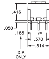
FRONT VIEW SINGLE AND DOUBLE POLE
