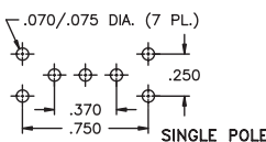
FRONT VIEW SINGLE POLE
