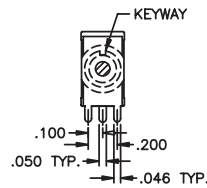
FRONT VIEW SINGLE POLE
