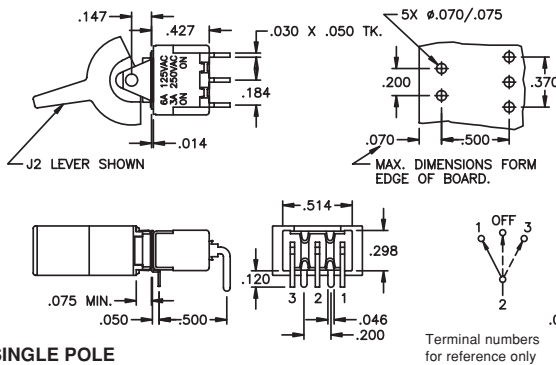
SINGLE POLE
