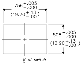
PANEL PIERCING
