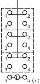
CONTACT CONFIGURATION
