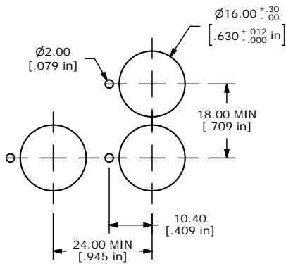
PANEL MOUNTING
