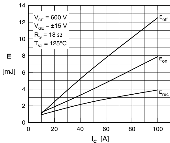
Fig. 5 Typical switching losses versus collector current impedance
