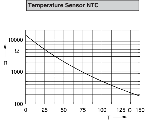
Fig. 24 Typ. thermistorresistance versus temperature
