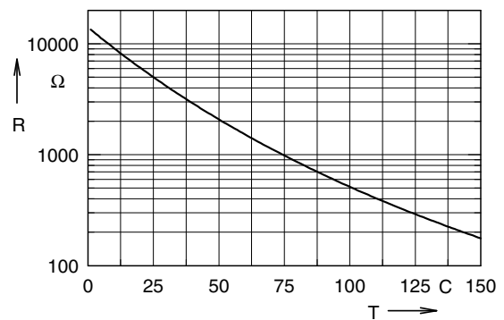
Fig. 24 Typ. thermistorresistance versus temperature
