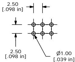
P.C. MOUNTING
