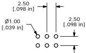
P.C. MOUNTING
