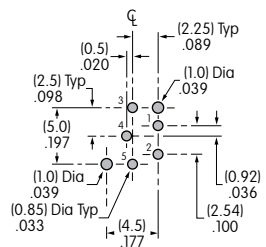
PCB Footprint
