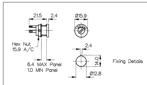
Connection Series 240V
