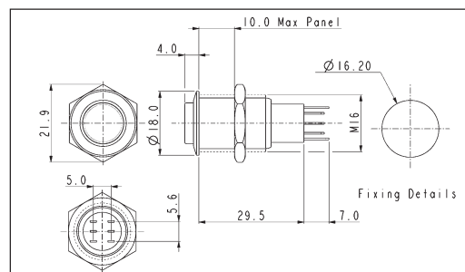
Contact Layout
