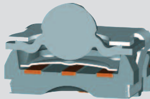
Sectional view of keyswitch
