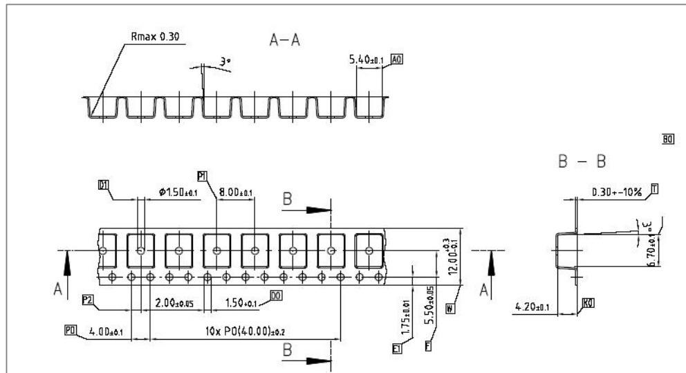
Tape and reel drawing:
