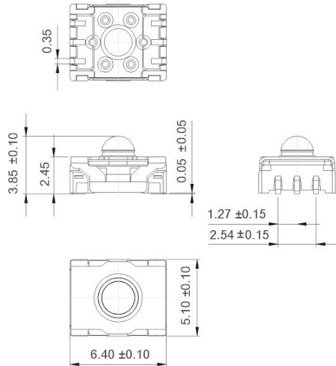
Dimensional drawing SMT standard version
