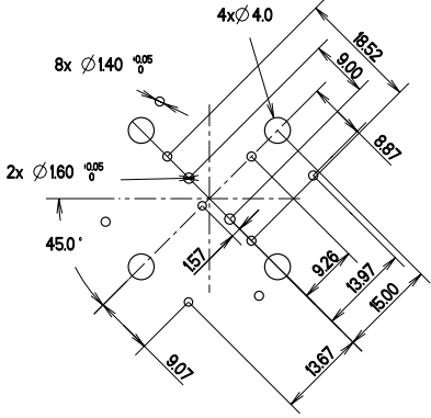
PCB LAYOUT
