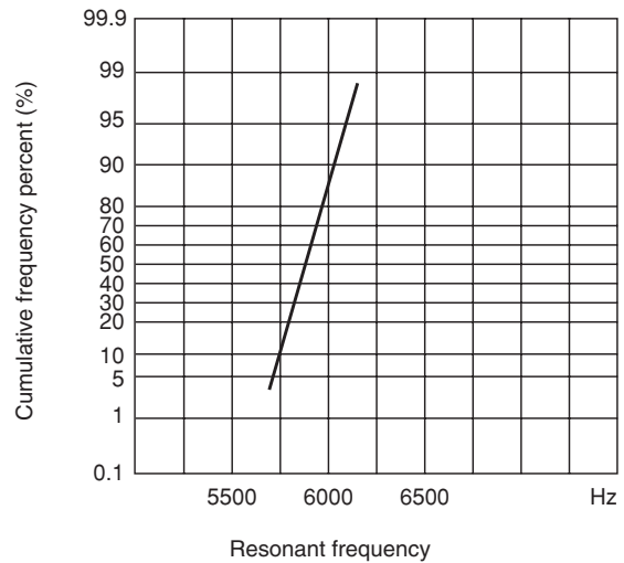
(4) Resonant frequency
