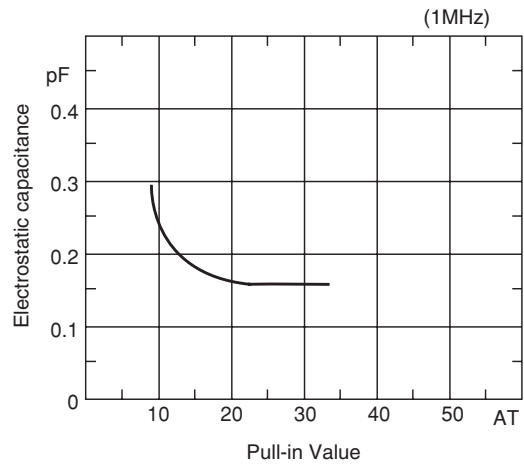
(5) Electrostatic capacitance
