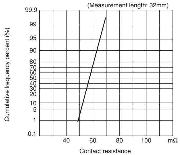
(2) Contact resistance
