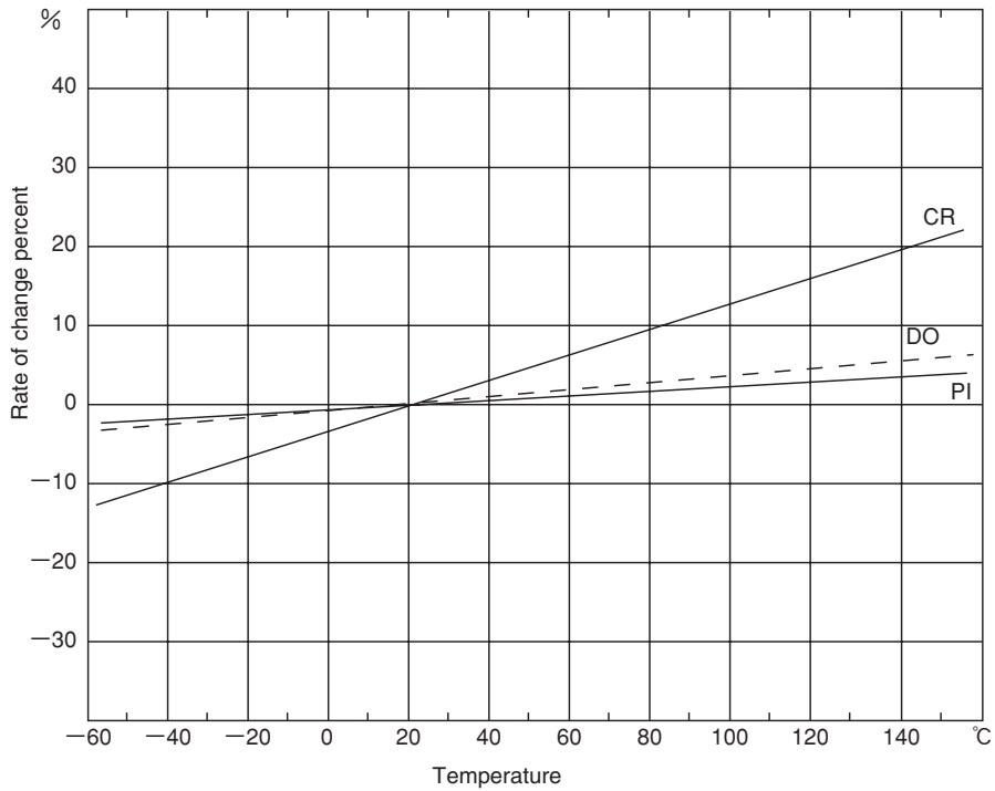
(1) Temperature characteristics
