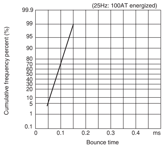
(2) Bounce time
