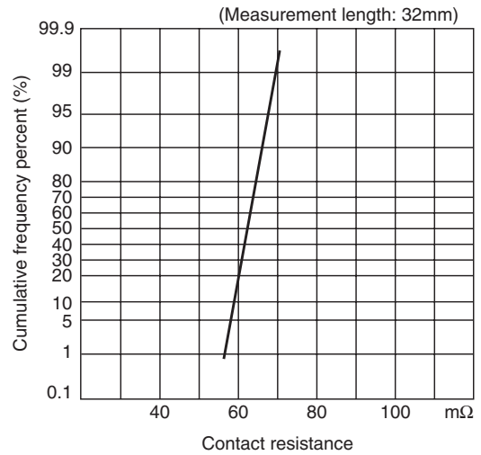
(2) Contact resistance
