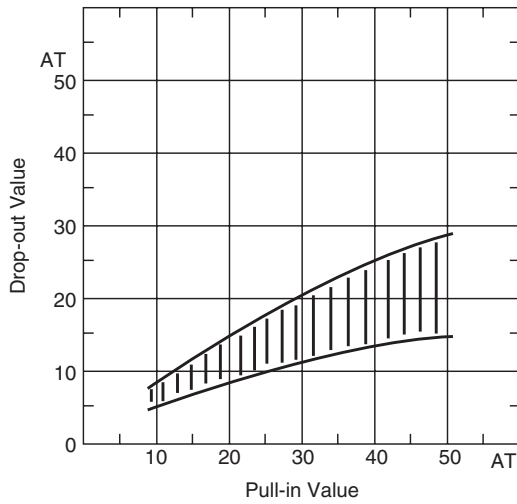
(1) Drop-out Value vs. Pull-in Value
