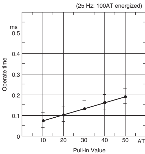
(1) Operate time
