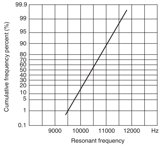
(4) Resonant frequency
