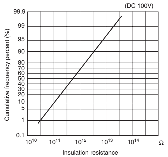
(4) Insulation resistance
