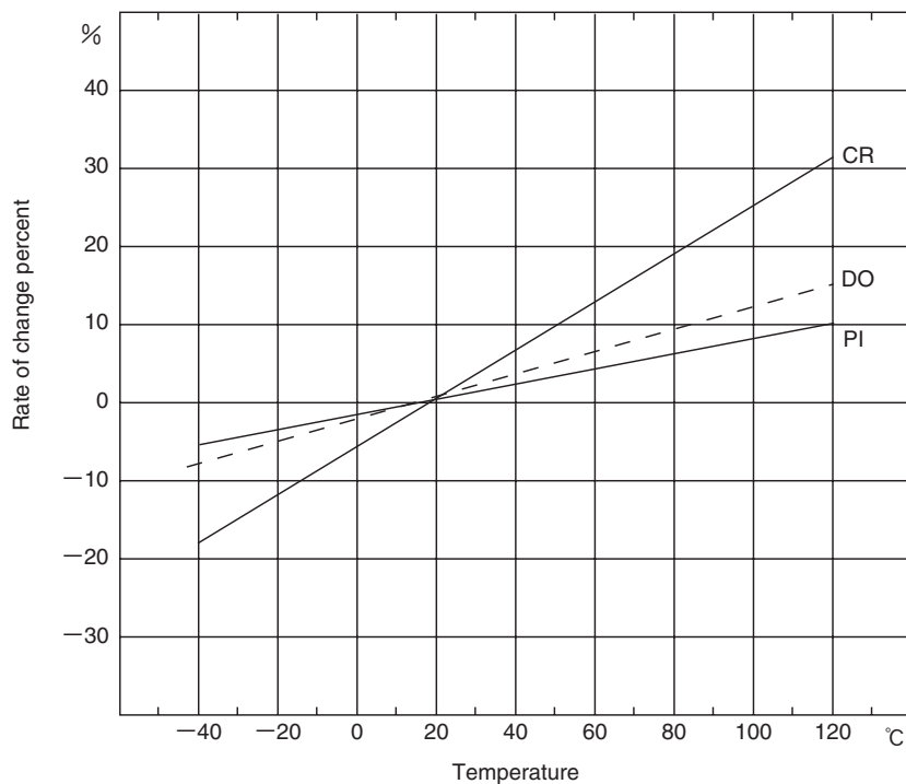
(1) Temperature characteristics
