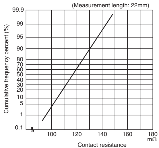
(2) Contact resistance
