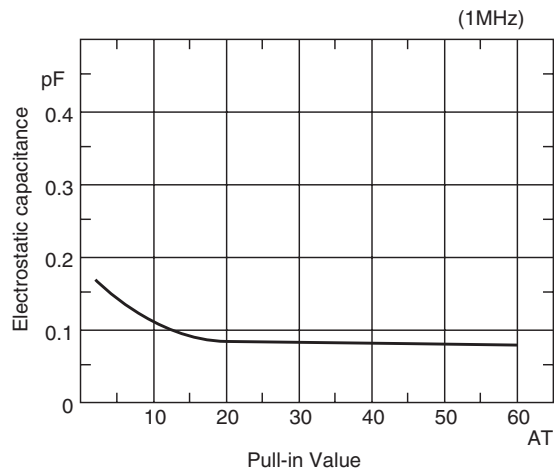
(5) Electrostatic capacitance
