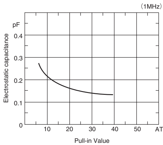
(5) Electrostatic capacitance
