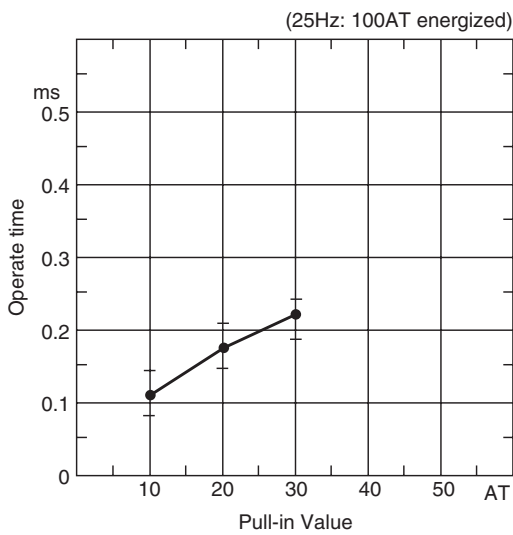
(1) Operate time
