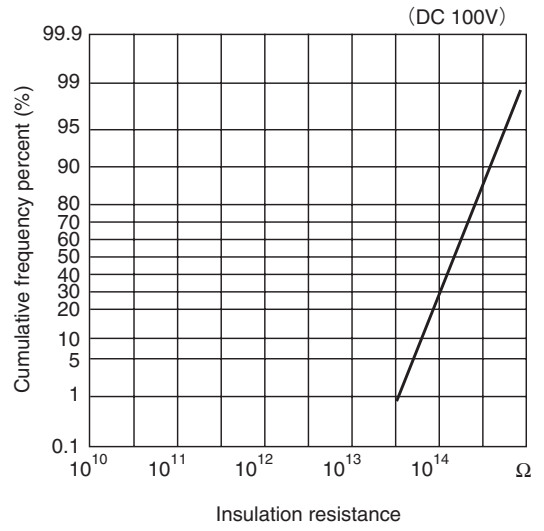
(4) Insulation resistance
