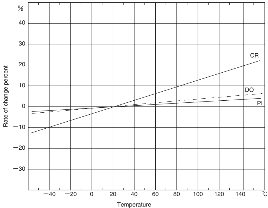
(1) Temperature characteristics
