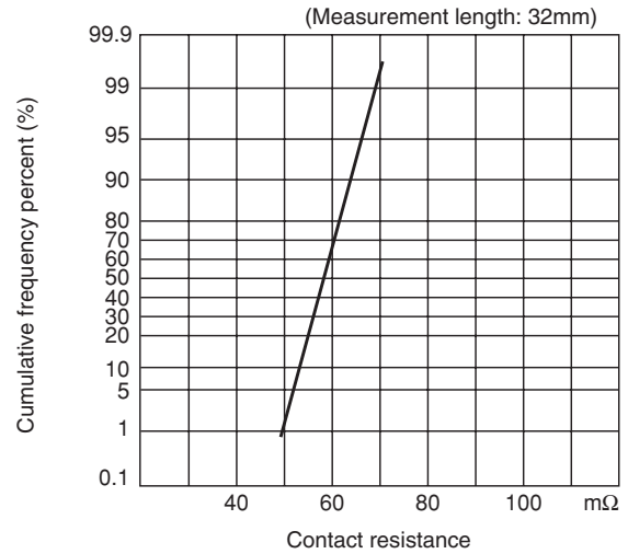
(2) Contact resistance
