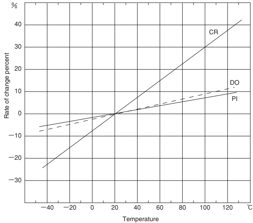
(1) Temperature characteristics
