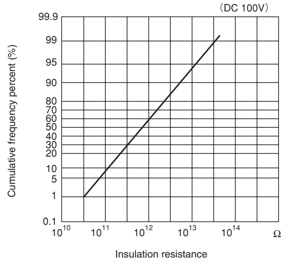
(4) Insulation resistance
