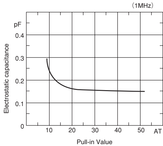
(5) Electrostatic capacitance
