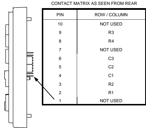
MATRIX VERSION SIDE VIEW & CONNECTION DETAILS
