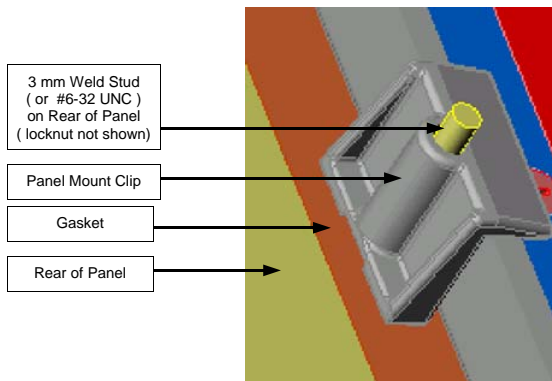
REAR VIEW SHOWING PANEL CLIP ARRANGEMENT
