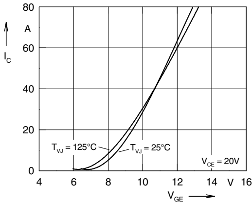
Fig. 9 Typ. transfer characteristics
