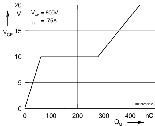
Fig. 4 Typ. turn on gate charge
