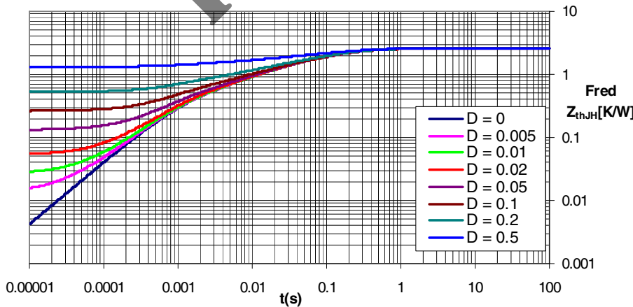
Transient thermal resistance junction to heatsink
