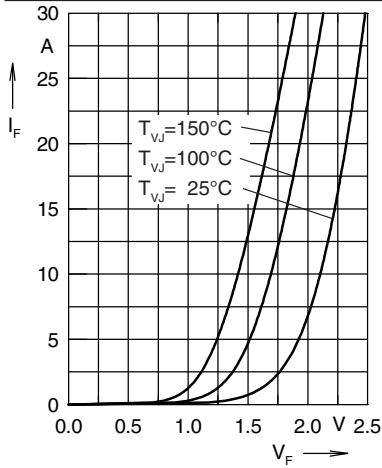
Forward current I_F versus V_F
