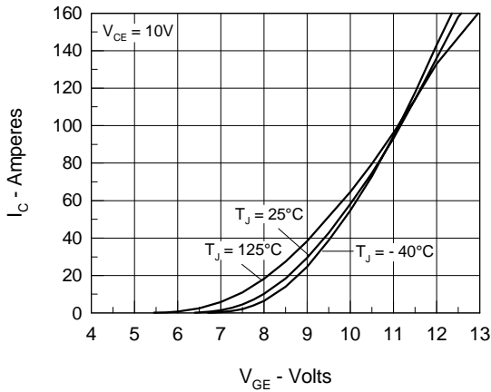
Fig.5 Input Admittance
