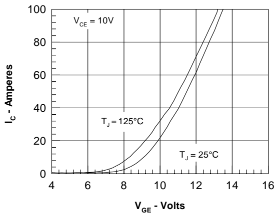
Figure 5. Admittance Curves
