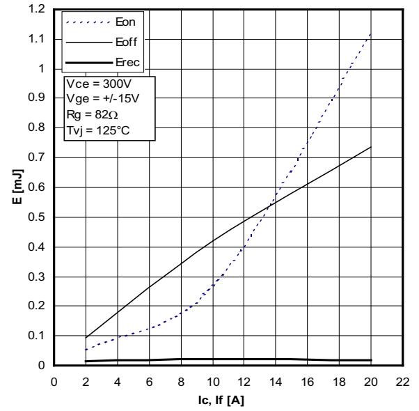
Typical switching energy versus collector current
