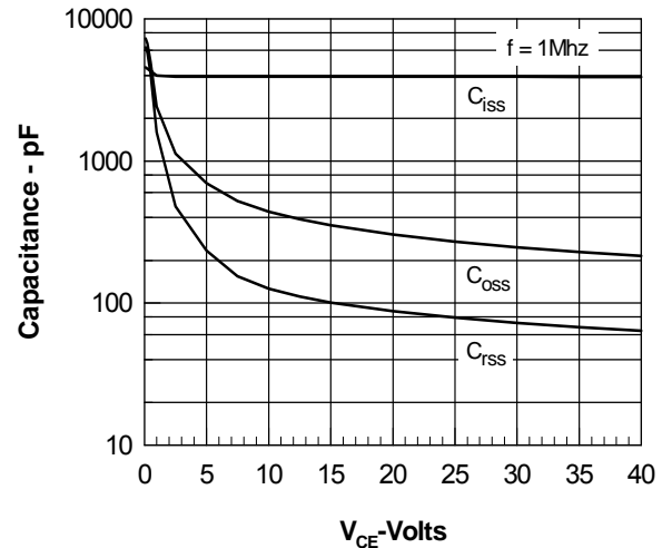
Figure 6. Capacitance Curves
