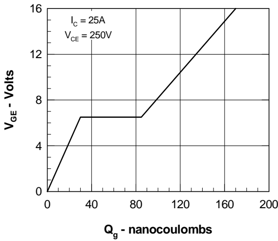
Figure 9. Gate Charge
