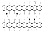
SCHEMATIC (POSITION 0)
