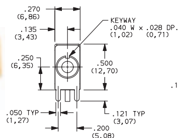
8121SD9AVGE SPDT
