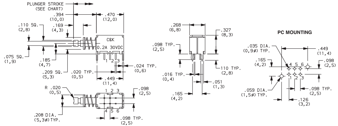
PN21SBSA03QE DPDT
