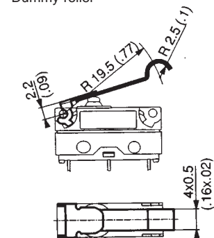
F Dummy roller
