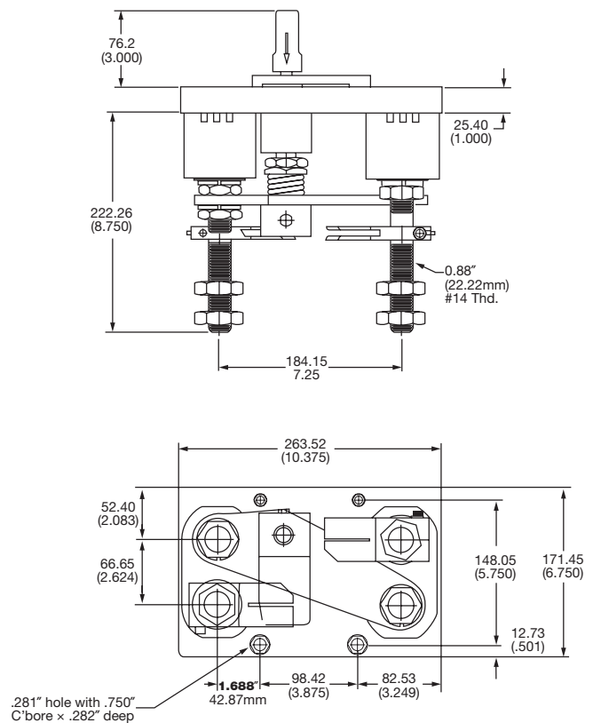
Dimensional Data 15200-609
