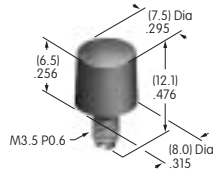
AT078 .315" Dia. Screw-on Cap Polystyrene Colors: A B C E F G H Series: MB20 SCB WB
