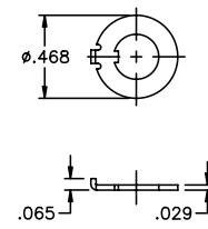
ANTI-ROTATE RING (LARGE) A158 Nickel plated brass 1/4
