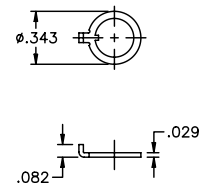
ANTI-ROTATE RING A107 Nickel plated brass 1/4
