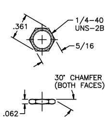
PANEL DRESS NUT A274 Nickel plated brass 1/4-40
