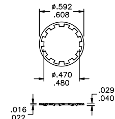
LOCKWASHER A466 Nickel plated steel 15/32
