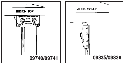
Figure 8. Installation of grounding blocks.
