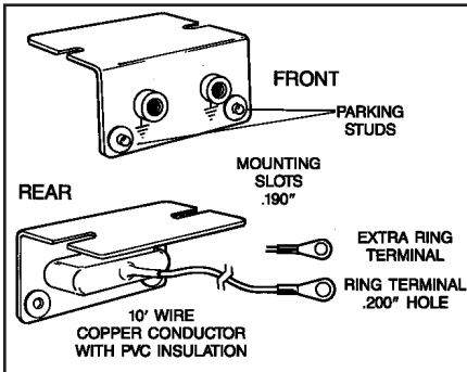
Figure 1. 09740/09741 wrist strap bench ground.
