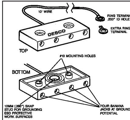
Figure 4. 09835/09836 quad common point ground
