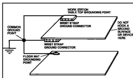
Figure 6. All elements at the ESD work station should be connected to the same common point ground, such as 09837 Multi Grounding Hub.
