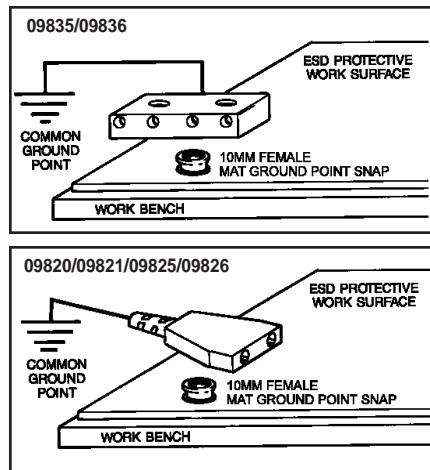
Figure 9. Installing the 09835/09836 and 09820/09821/09825/09826 as a common point ground cord for a work surface.
