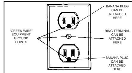
Figure 7. Recommended grounding point.
