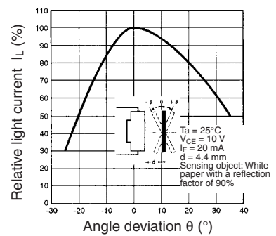
Sensing Angle Characteristics (Typical)
